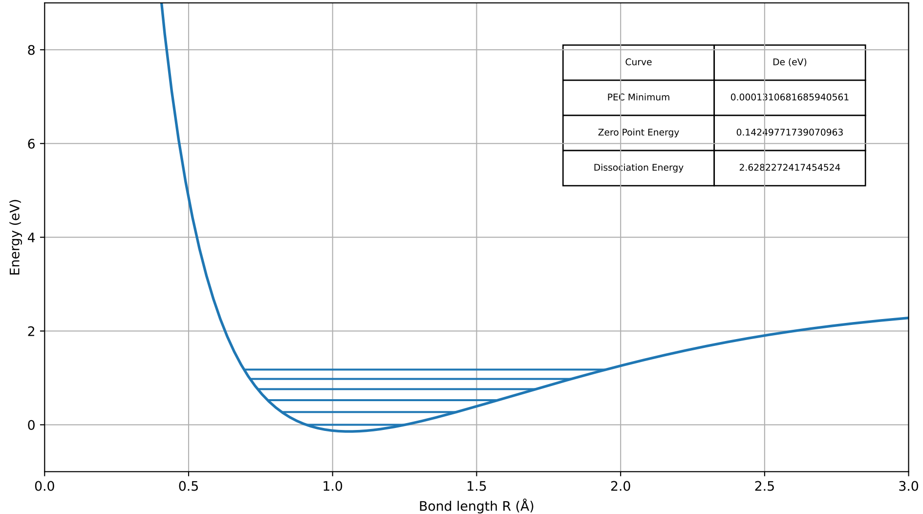
\text{H}_2^+ Ground State PEC and Vibrational Energies
